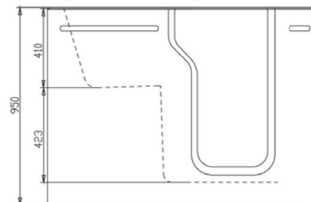
Front view for Stamford Range Right hand model shown
