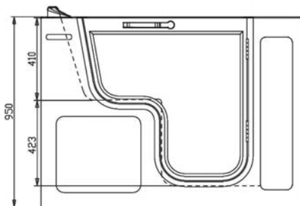
Front view for Oakham Range Right hand model shown
